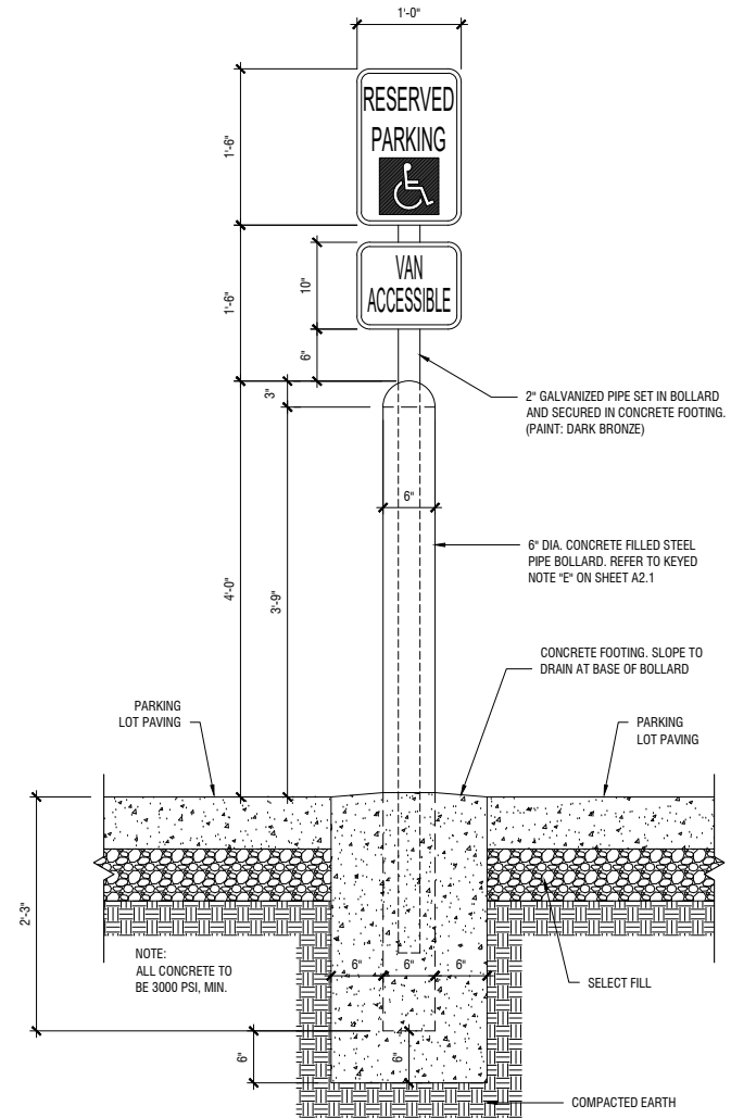
ADA SIGN DETAIL ON POST
