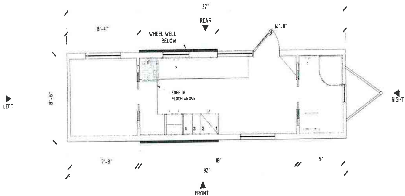
1 LOWER LEVEL SCALE \frac{1}{4}"=1'-0"
