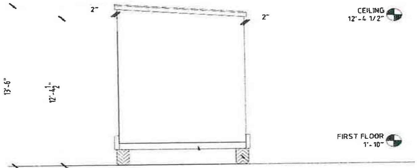
LEFT ELEVATION SCALE \frac{1}{4}" = 1'-0"
