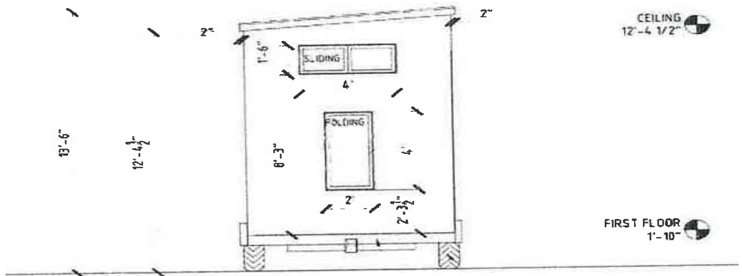
RIGHT ELEVATION SCALE \frac{1}{4}" = 1'-0"
