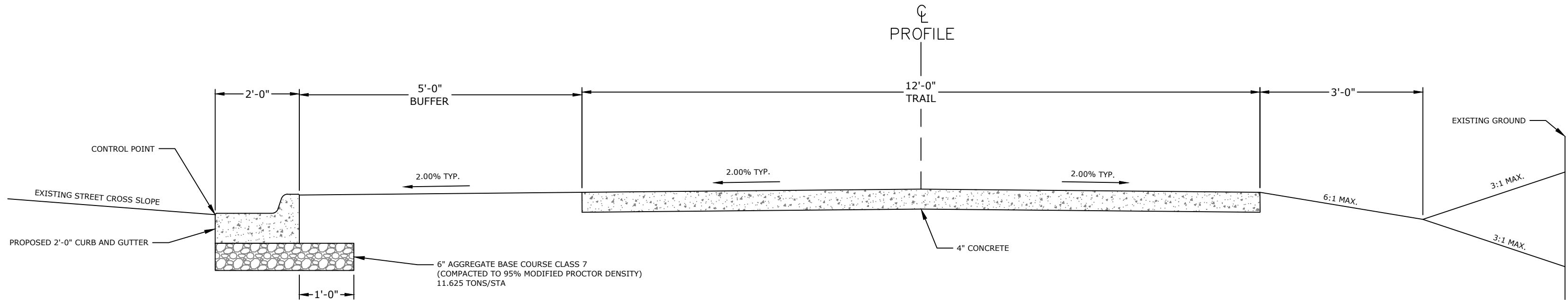
TRAIL WITH 5' BUFFER ON PROPOSED BACK OF CURB DETAIL (WITH GUTTER) N.T.S.
