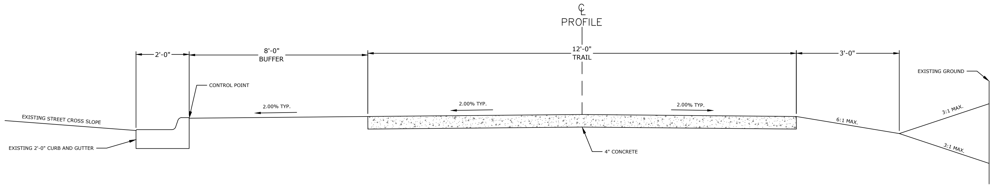
TRAIL WITH 8' BUFFER ON EXISTING BACK OF CURB DETAIL (WITH GUTTER) N.T.S.
