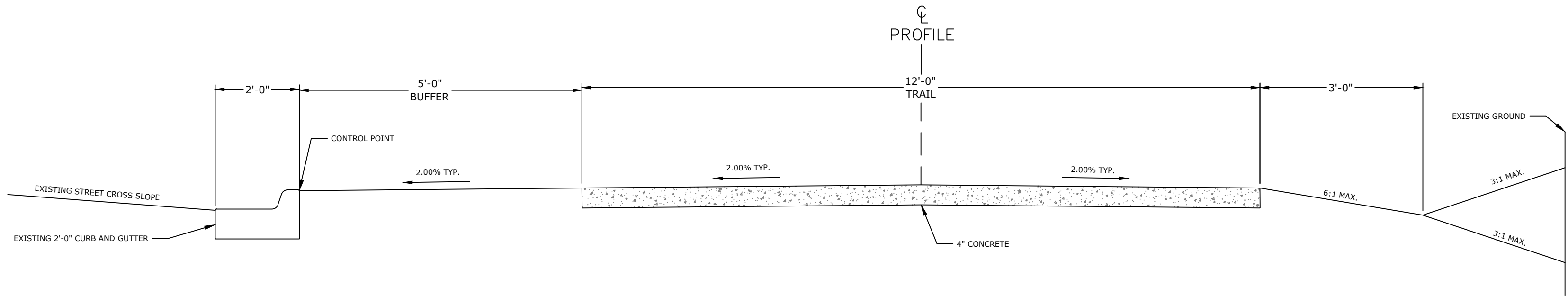
TRAIL WITH 5' BUFFER ON EXISTING BACK OF CURB DETAIL (WITH GUTTER) N.T.S.
