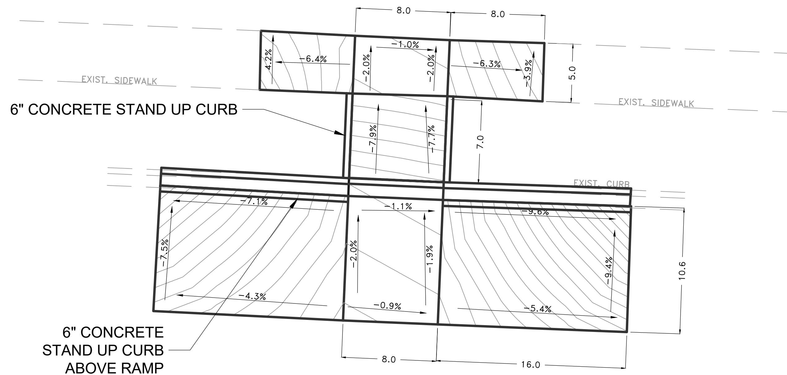
PROPOSED SLOPES
