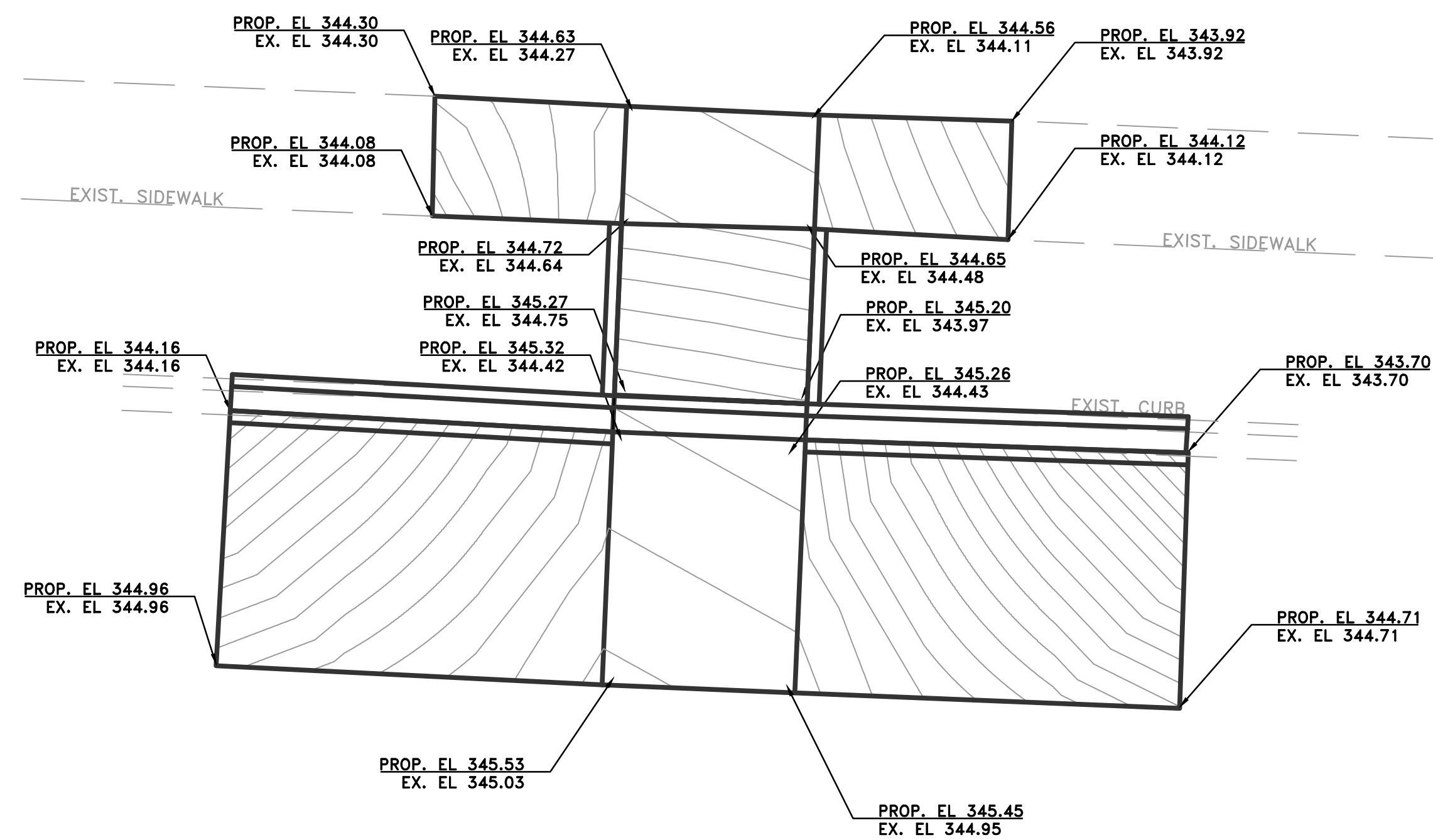
PROPOSED ELEVATIONS
