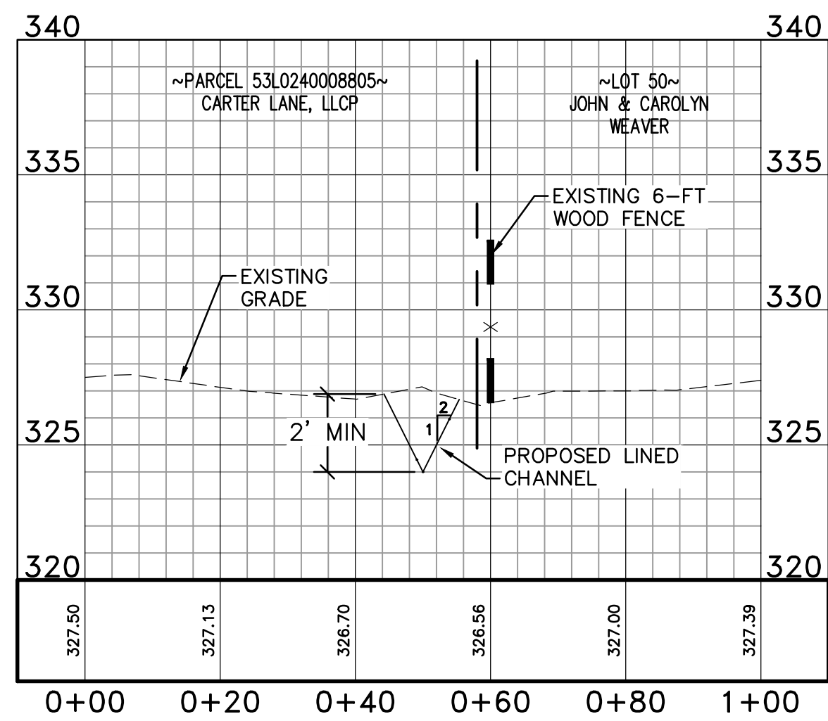
TYPICAL SECTION STA 13+80
