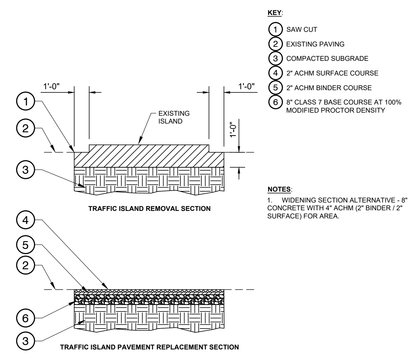
1 CHENAL TRAFFIC ISLAND REMOVAL DETAIL 1/4" = 1'-0"
