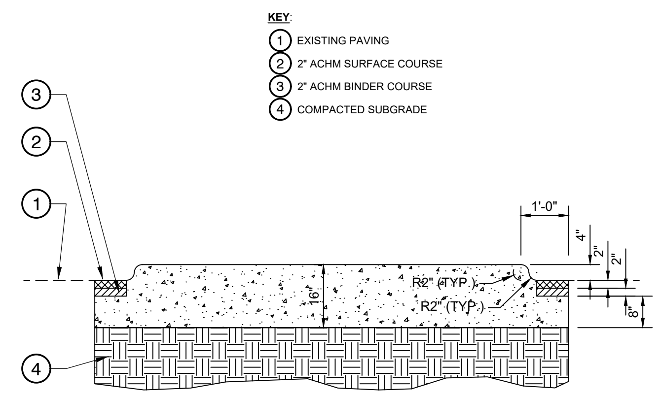
2 CHENAL TRAFFIC ISLAND DETAIL NTS
